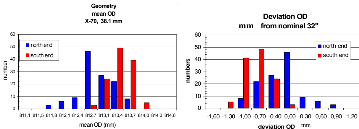
Figure 11: Deviation of the outside diameter in mm and in % of nominal ID for 38.1 mm wall
