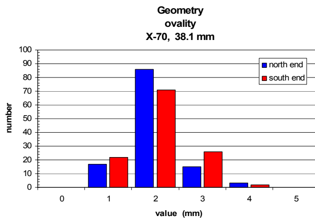
Figure 12: Out of roundness (OOR) values measured at orders with 38 mm wall
