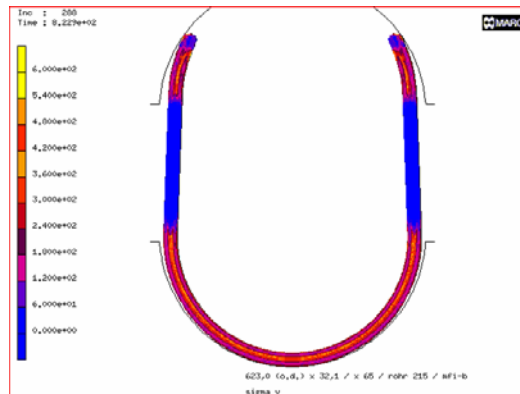
Figure 06: FEA Simulation of the O-ing Process
